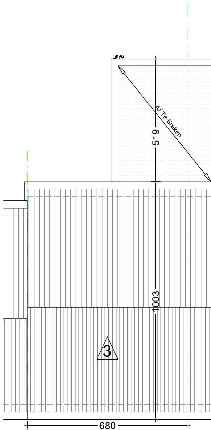
BT DAKENPLAN 1/100
